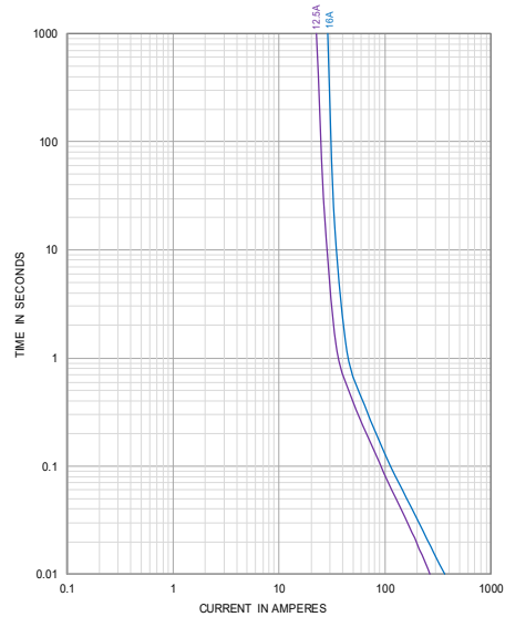
Average Time Current (I-T) Curves
